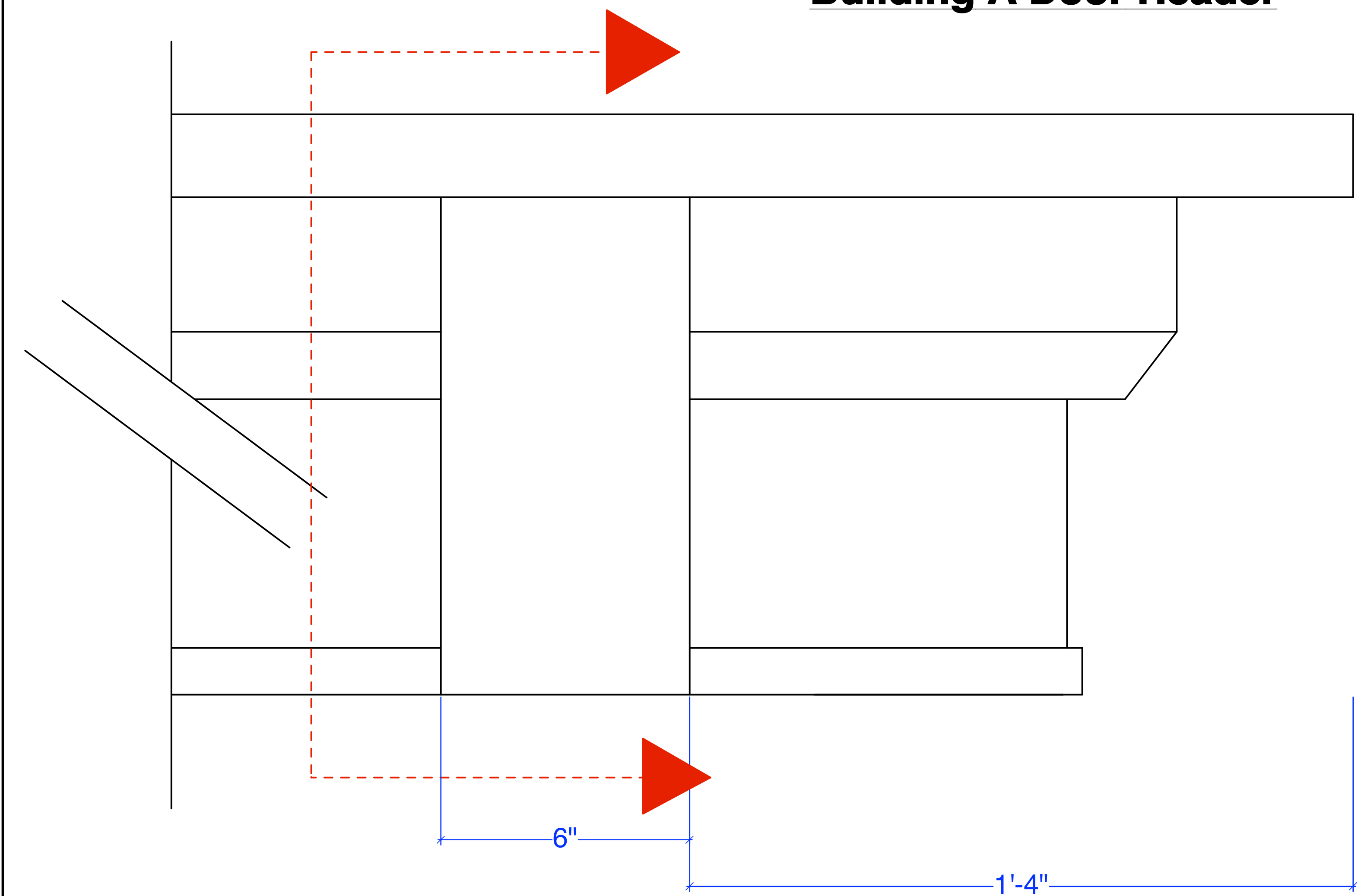
Building A Door Header
