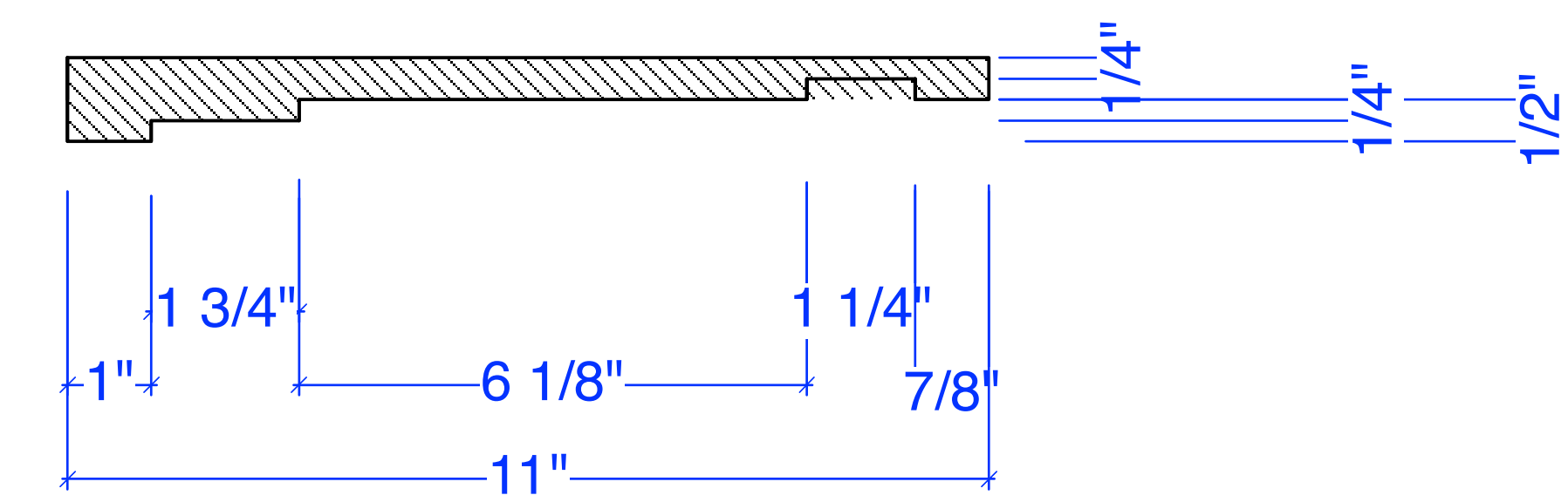
Building A Door Surround
