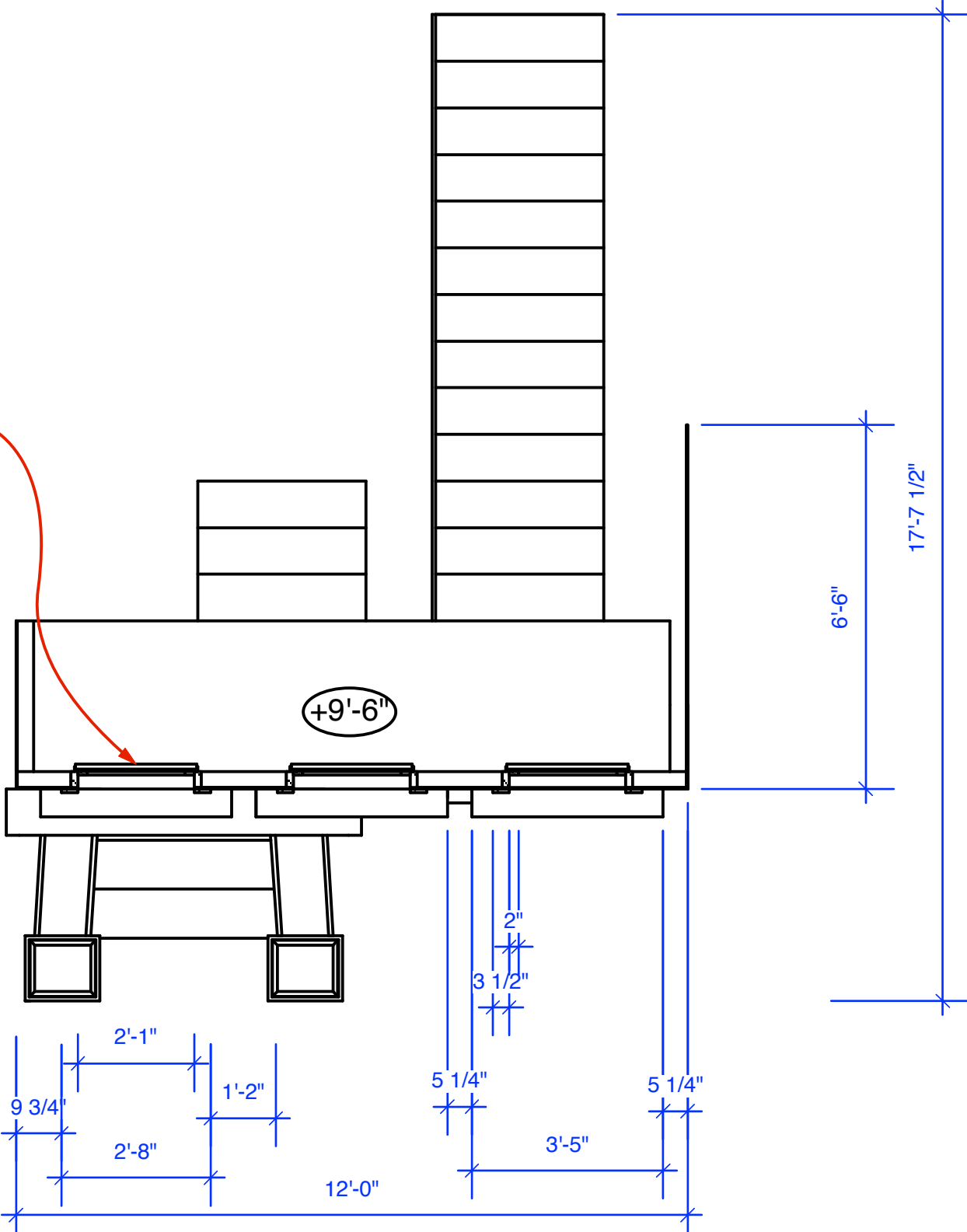
TOP SECTION VIEW
