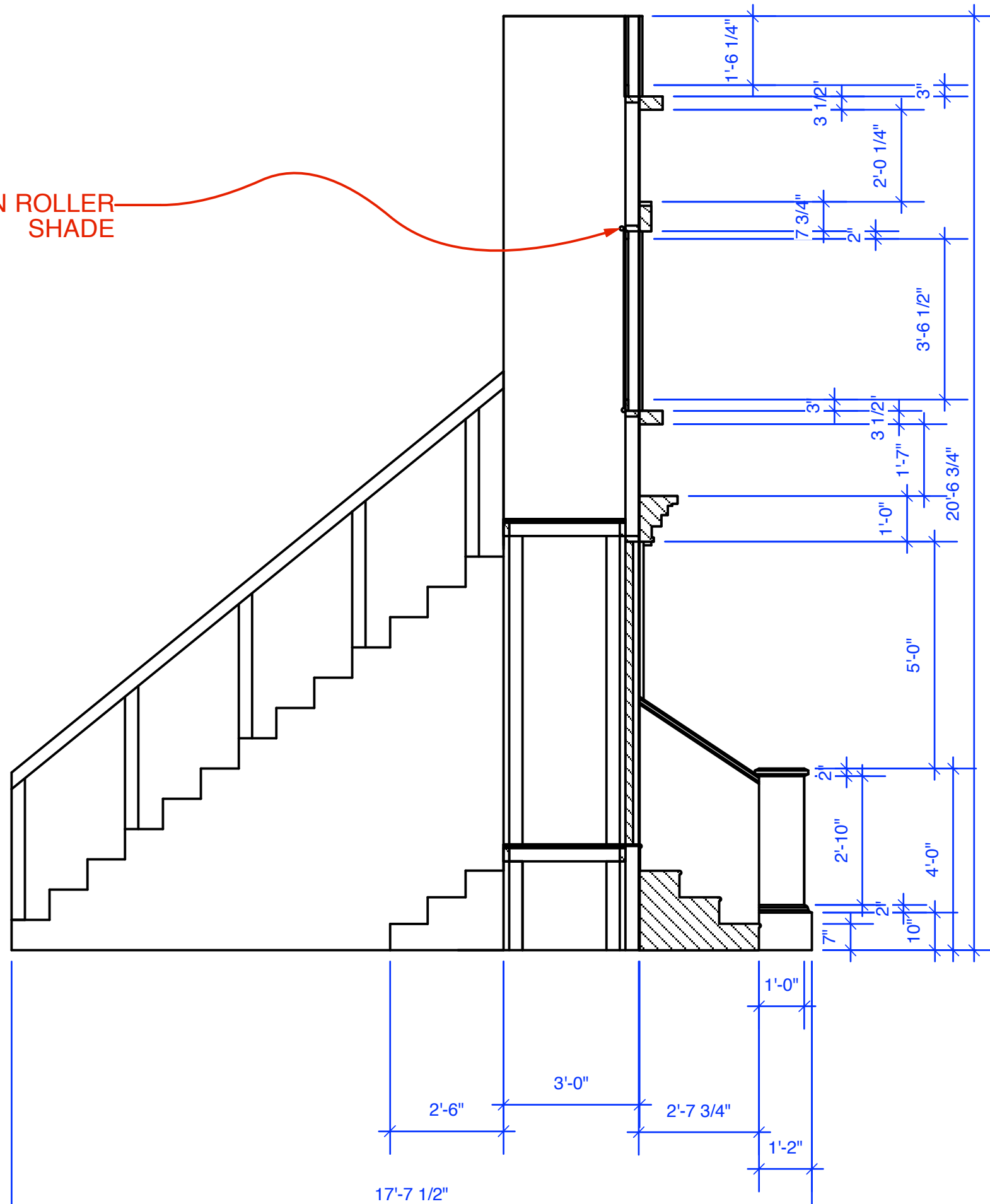
SIDE SECTION VIEW
