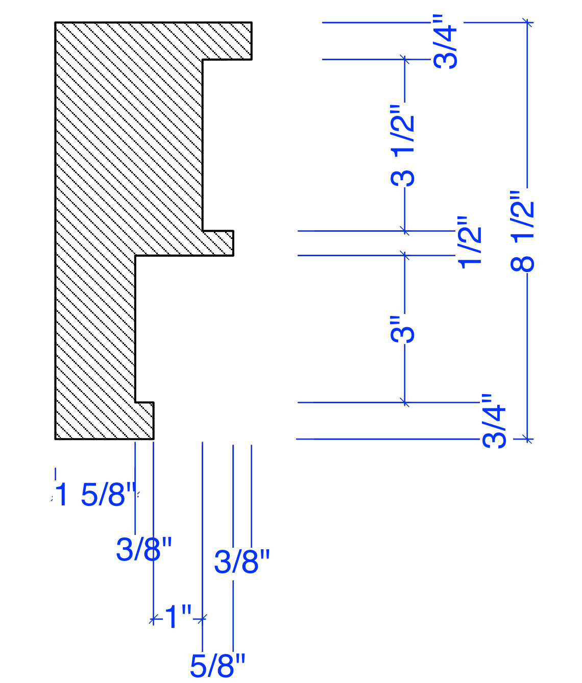
Building C Door Header
